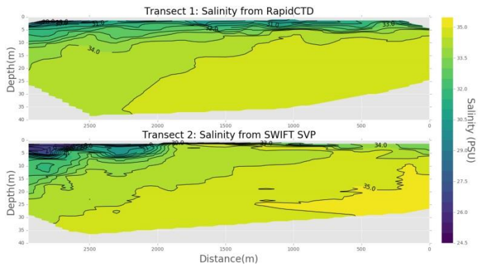
Figure 5: Salinity transects
