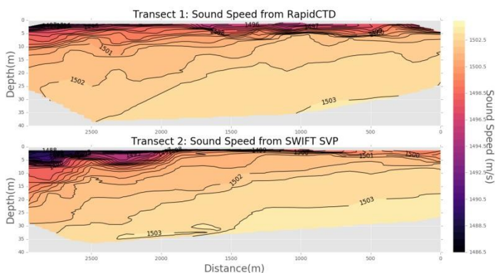
Figure 7: Sound speed transects
