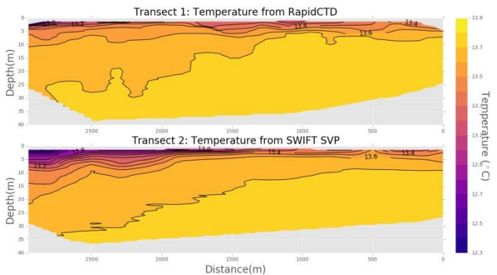
Figure 6: Temperature transects
