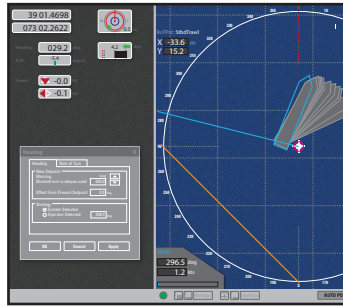
Dynamic Positioning
