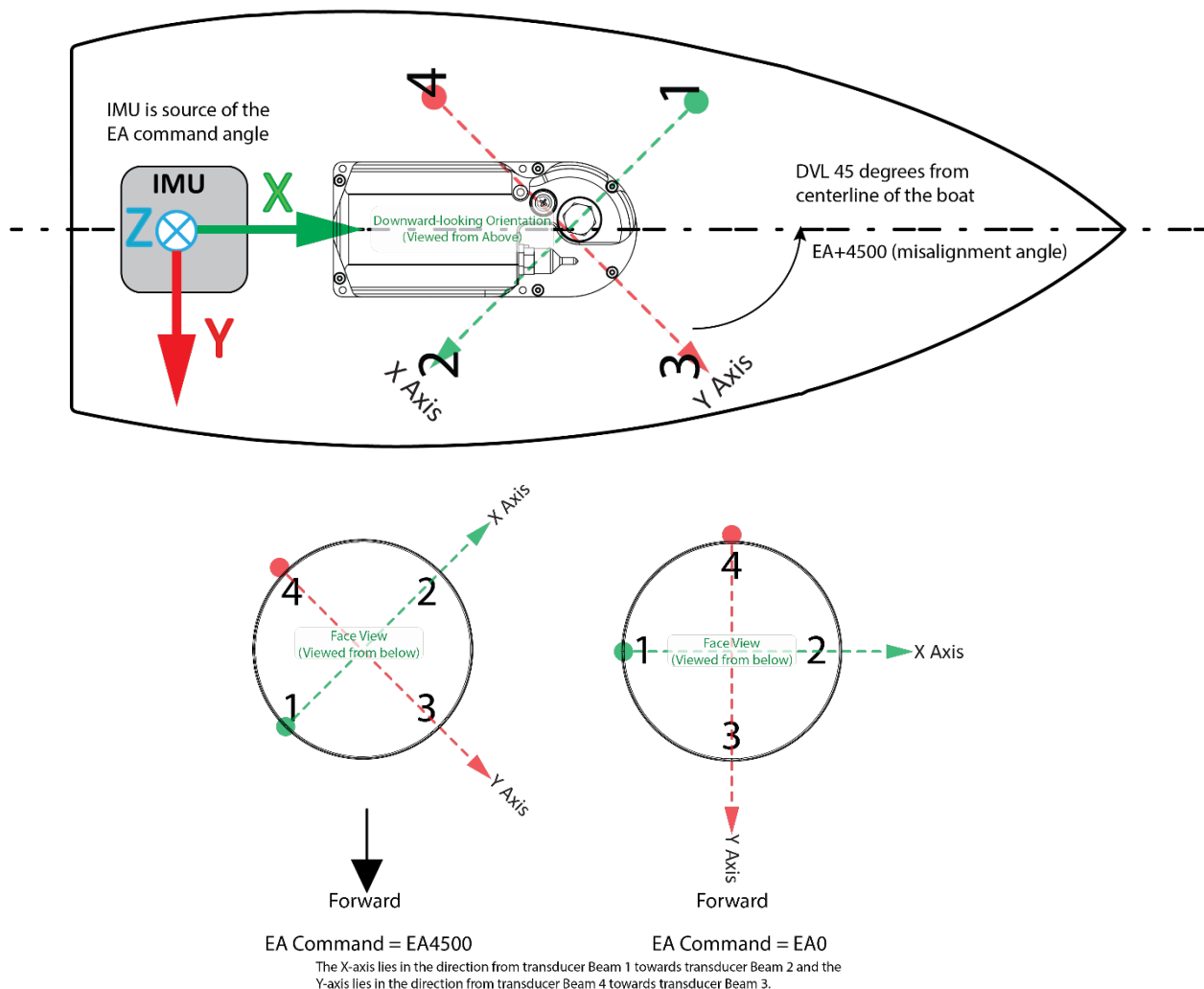
Figure 23. Transducer Alignment Reference Points
