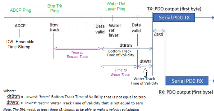
Figure 49. No Trigger Timing
