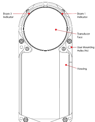
Figure 28. Transducer View
