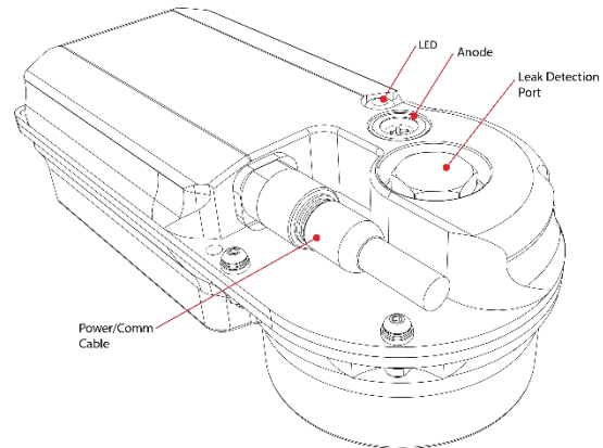
Figure 29. Top View
