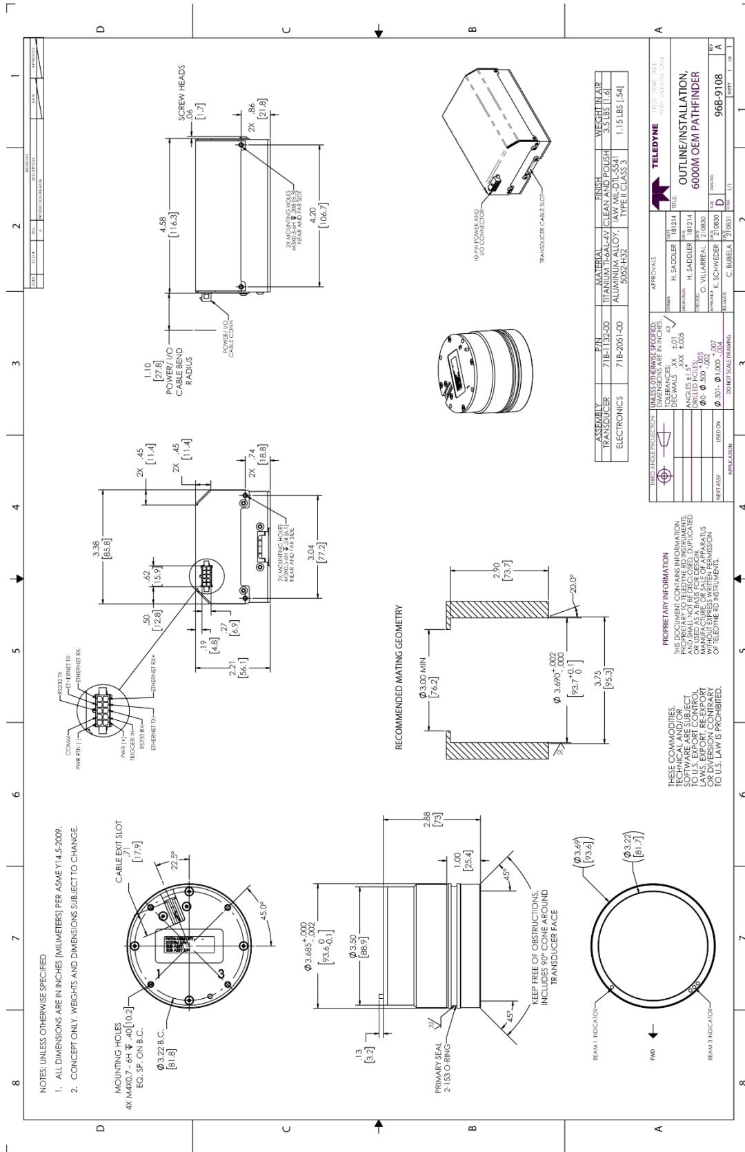
Figure 33. Outline Installation Drawing – OEM 6000 meter
