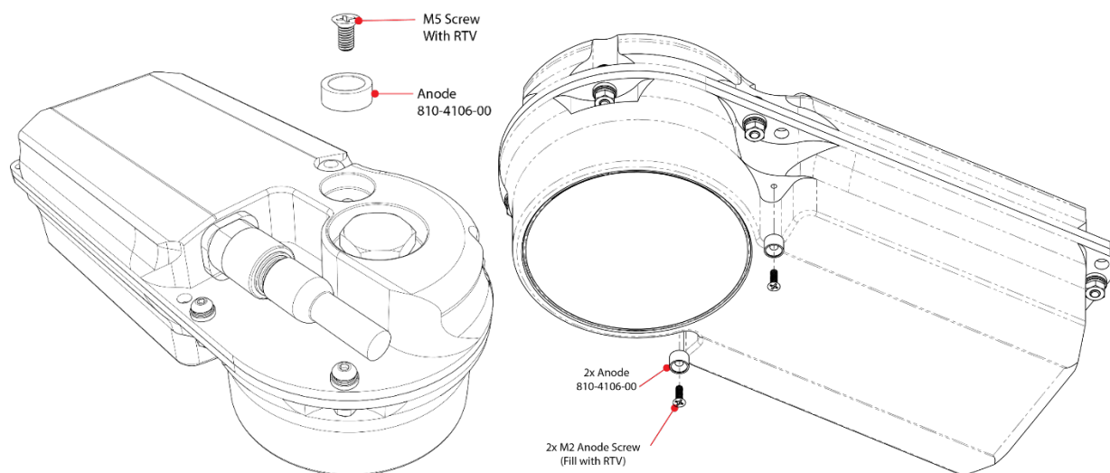
Figure 30. Replacing an Anode
