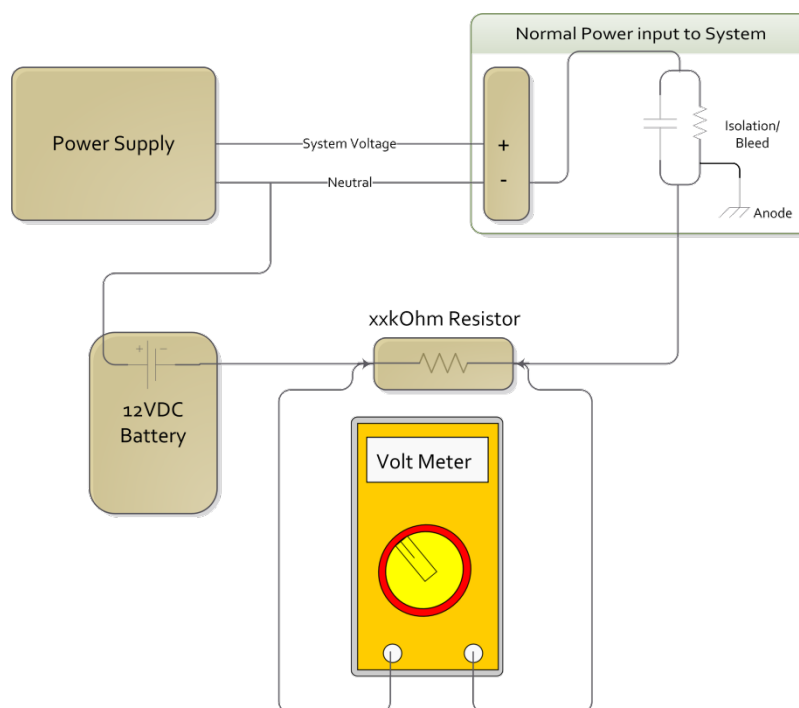
Figure 26. Ground Fault Current Check
