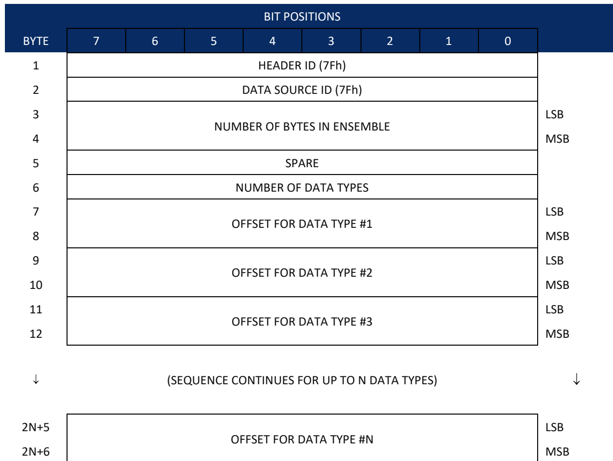
Figure 38. Binary Header Data Format
