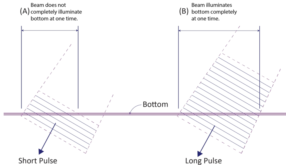
Figure 17. Short Pulse versus Long Pulse
