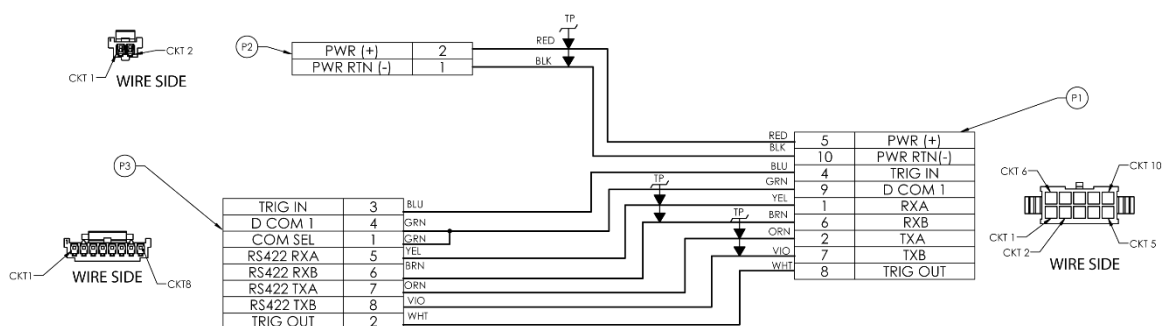
Figure 14. Pathfinder OEM Power/Comm 73B-2382-01 (RS-422)
