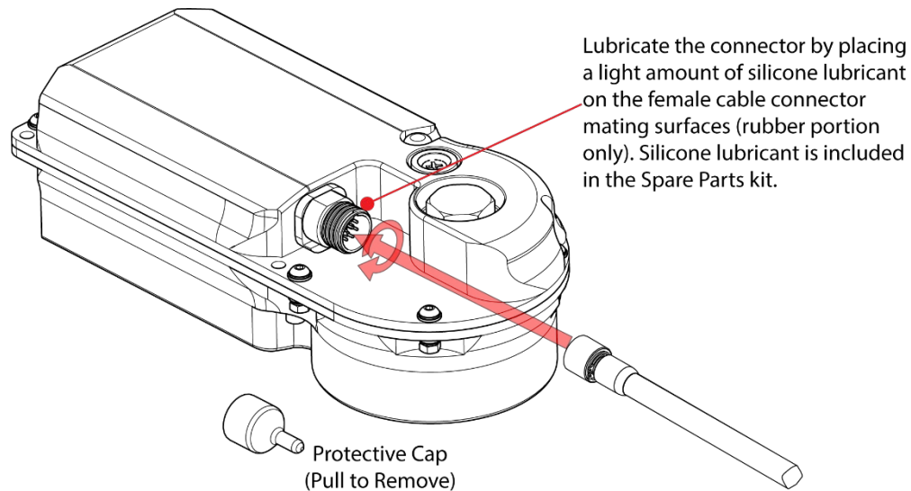
Figure 4. Connecting the Cable
