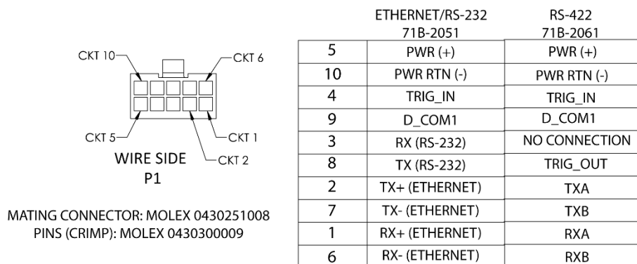
Figure 15. Pathfinder OEM Power/Comm 10-Pin Connector Pinout
