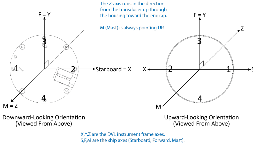
Figure 21. Pathfinder Ship Coordinates (OEM Transducer Shown)
