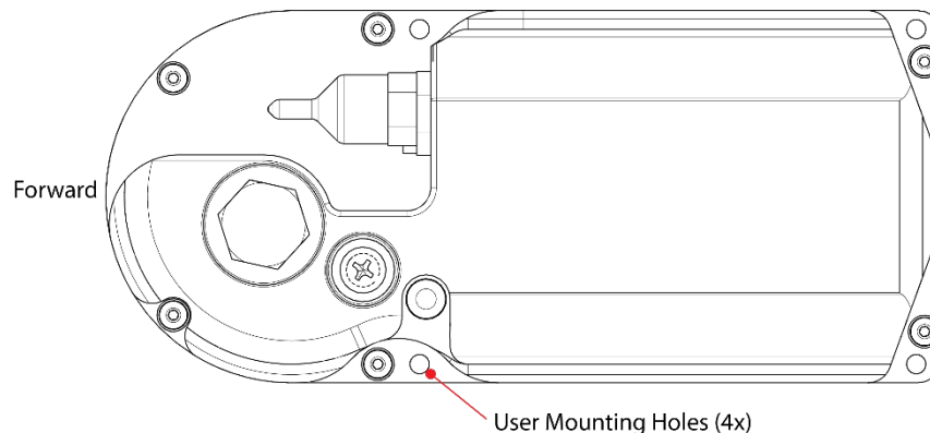
Figure 24. End-Cap view of the transducer showing mounting holes
