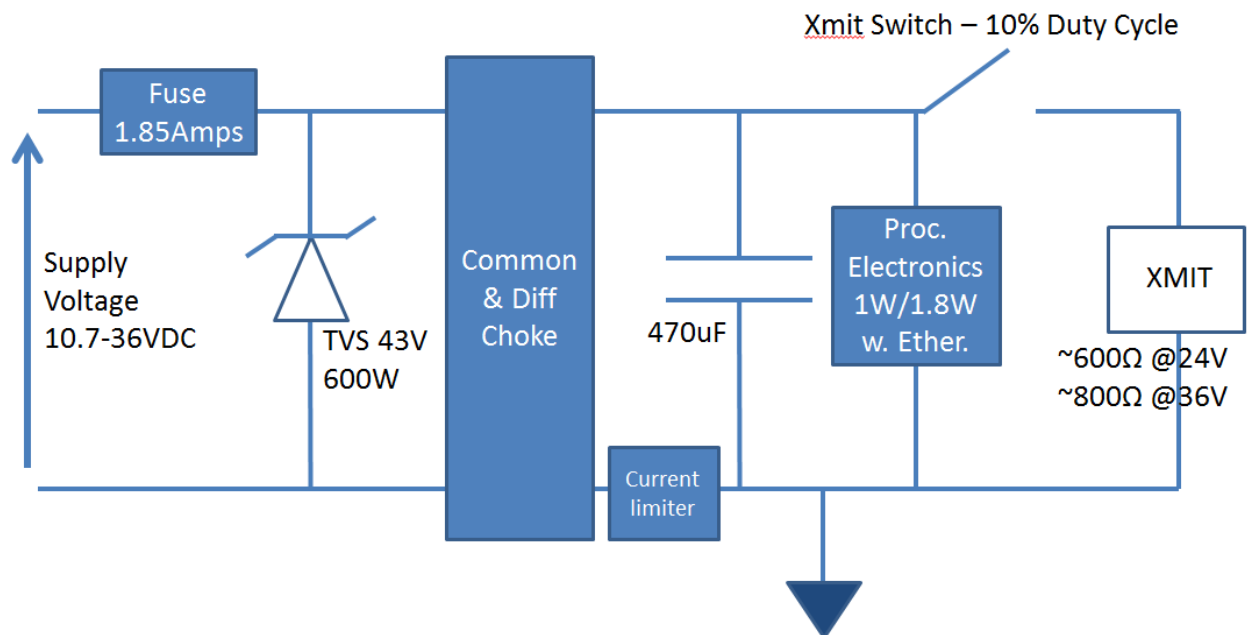
Figure 27. Pathfinder Power Circuit
