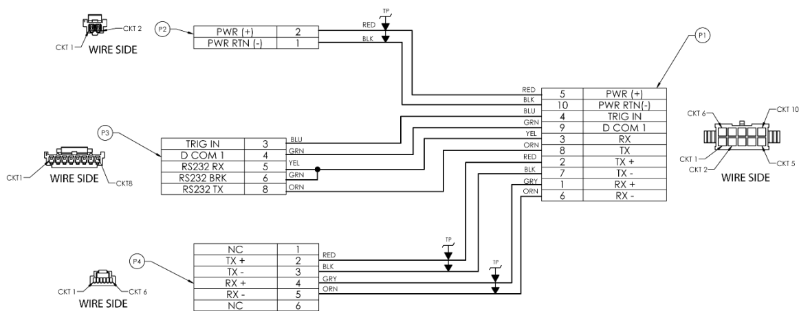
Figure 13. Pathfinder OEM Power/Comm 73B-2382-00 (Ethernet/RS-232)
