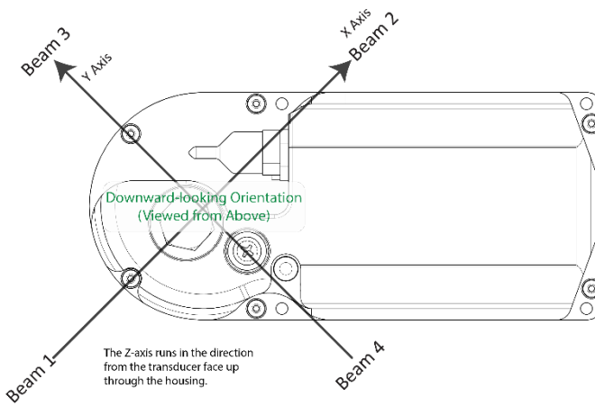
Figure 20. X, Y, and Z Velocities (ROV version shown)
