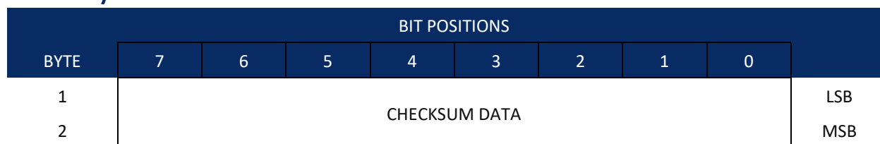
Figure 52. Binary Checksum Data Format
